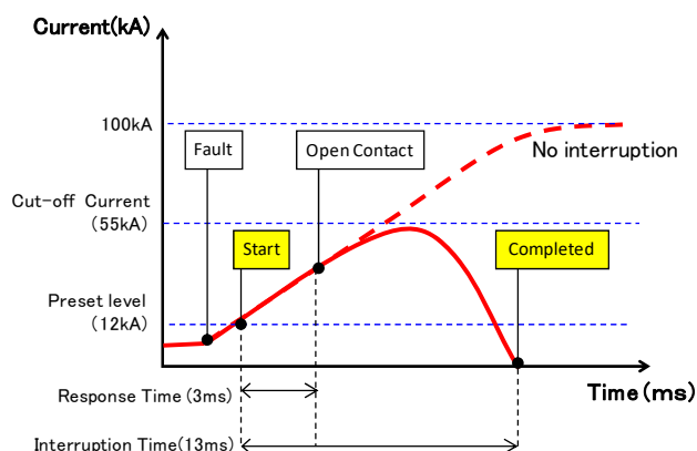
Waveform of a short circuit current interruption
