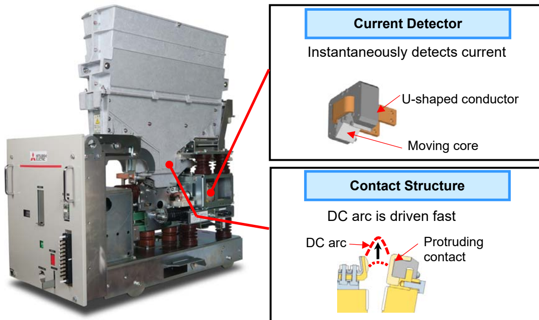
New High-speed Circuit Breaker
